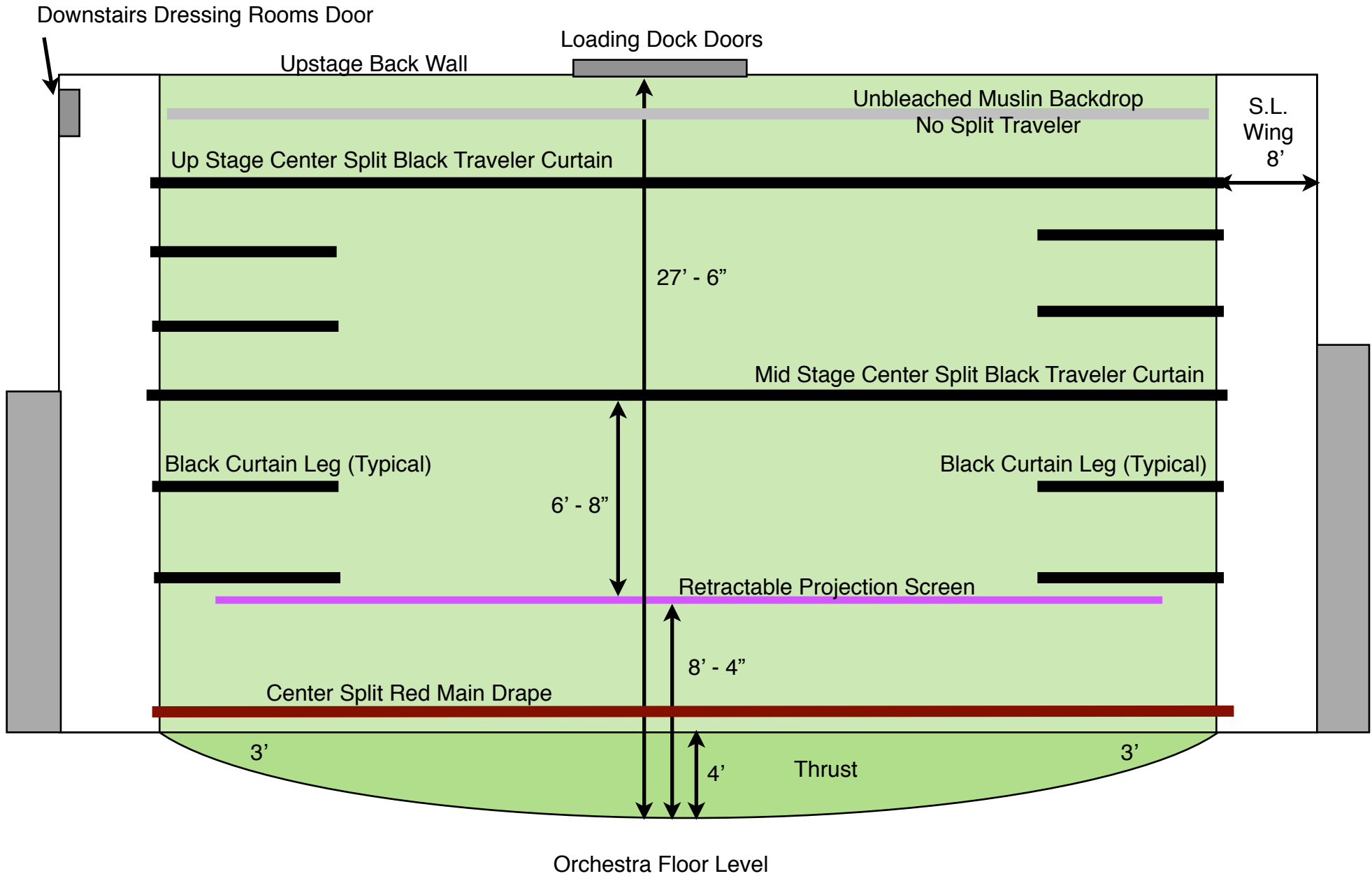
Star Hall Moab Utah - Stage Curtains Detail - Not To Scale
